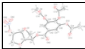
Fig. 1. Molecular structure of the title compound (I), showing the atom labeling scheme. Displacement ellipsoids are drawn at the 30% probability level. H atoms are represented as small spheres of arbitrary radii.
